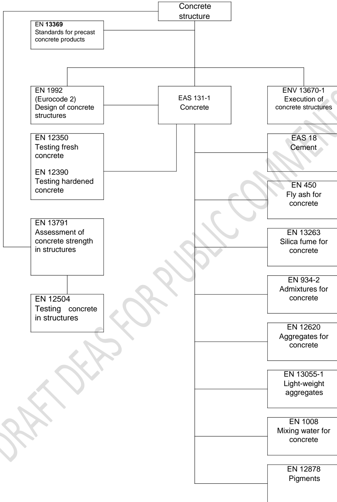
Figure 1 – Relationship between EAS 131-1 and standards for design and execution, standards for constituent materials and test standards
